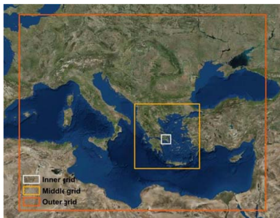
Fig. 5 The system of nested grids used for the CAMx simulations
