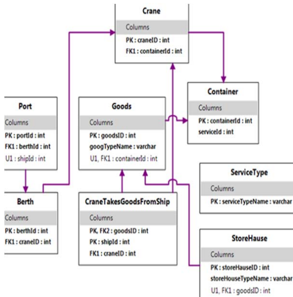
Fig. 5 Conceptual Scheme with ERM model
