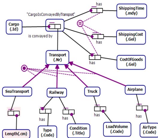
Fig. 2 Fragment of a conceptual scheme with ORM
