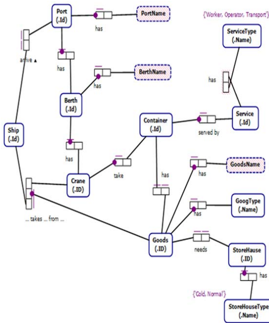
Fig. 3 ORM with Objects and Predicates
