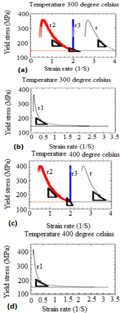
Fig. 1 (a)-(d) Plots of yield stress and strain rate at different temperatures and SRS calculated at the slopes of the grain size variants. Some of the plots of yield stress and strain rate at different temperature and SRS calculated at the slopes of the grain size variants are found in [19]
