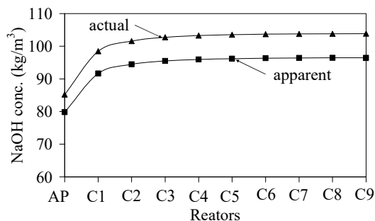
Fig. 3 NaOH concentration
