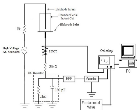
Fig. 5 Schematic circuit for PD measurement
