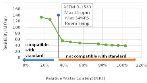
Fig. 9 Dependence of resistivity on water content
