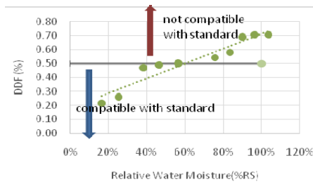
Fig. 7 Dependence of Dissipation Factor on Water content
