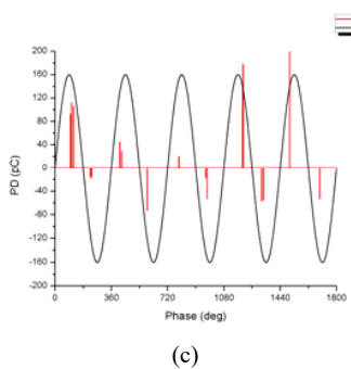
Fig. 15 PD pulse sequences of Sample (a) M03 (b) M05 and (c) M10 at applied voltage of 11 kV
