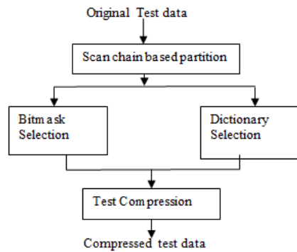
Fig. 3 Bitmask based code compression technique
