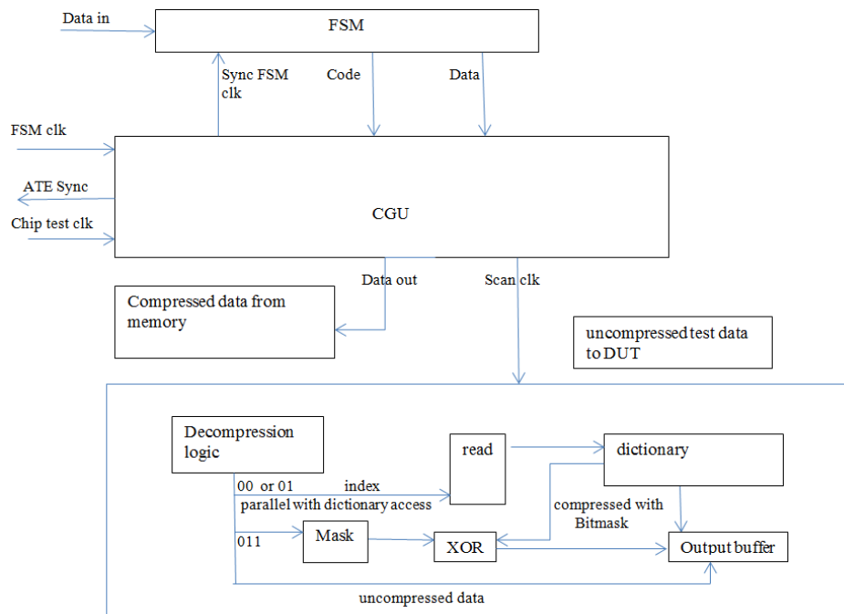
Fig. 6 Decompression architecture
