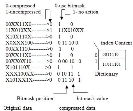
Fig. 4 Compression using bitmask and dictionary
