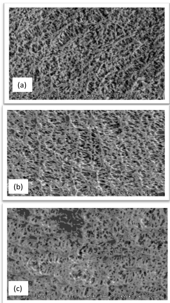
Fig. 4 SEM images of non-aged sample (a); aged samples at 80% RH-80°C for 144 hours (b); and 456 hours (c) of the e-PTFE
