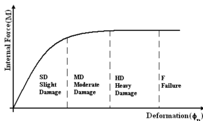
Fig. 3 Damage levels of a section
