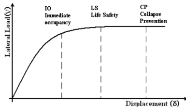
Fig. 2 Performance levels of a structure
