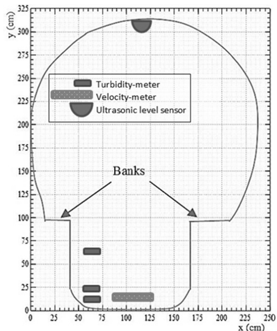
Fig. 1 Sewer Section Details and Measurement Equipment Position
