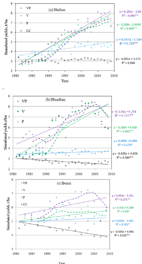
Fig. 4 The simulated yields of four simulating experiments including change of variety and planting date ( Y_{VP} , purple line), variety change ( Y_V , green line), planting date change ( Y_P , blue line), and only climate change ( Y_{CC} , black line) from 1981 to 2009 at Hailun (a), Huadian (b) and Benxi (c) stations. Line trend (solid line) and six years moving average line (dot line). *, ** is significant at P < 0.05 and P < 0.01 level, respectively
