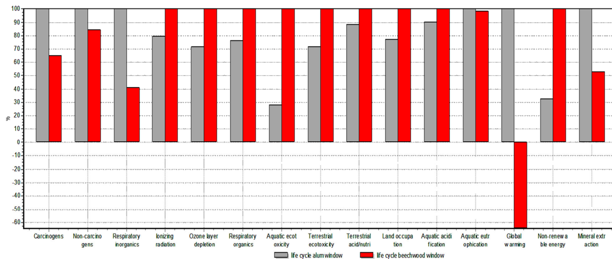
Fig. 12 Characterization factors for aluminum and beech wood windows
