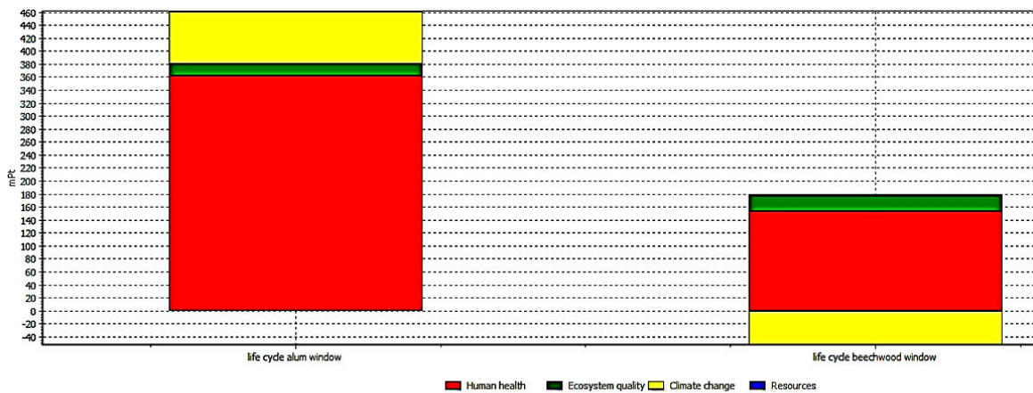
Comparing 1 p 'life cycle alum window' with 1 p 'life cycle beechwood window'; Method: IMPACT 2002+ V2.12 / IMPACT 2002+ / Single score
