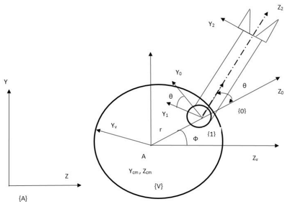
Fig. 4 Schematic diagram of 1 DOF flexible manipulator
