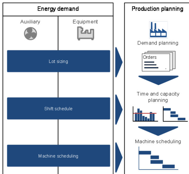
Fig. 3 Planning methods and power demand
