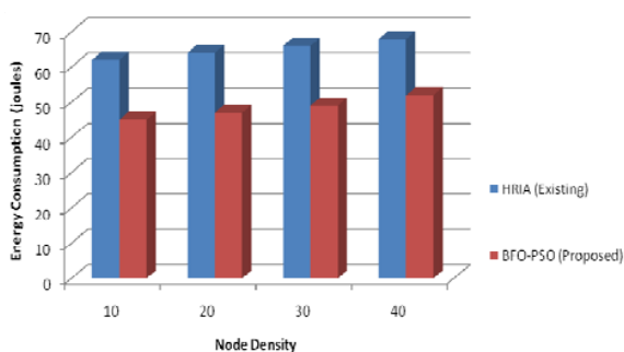
Fig. 4 Node Density Vs Energy Consumption (joules)
