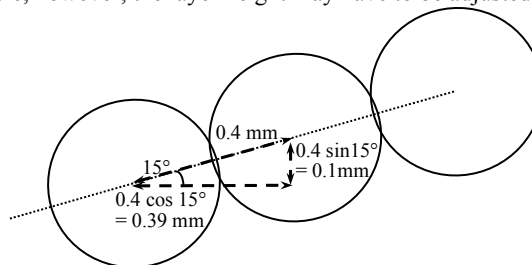
Fig. 7 Decision of layer height
