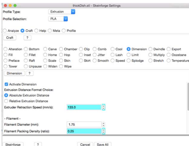
(b) Skeinforge—changing filament packing density
