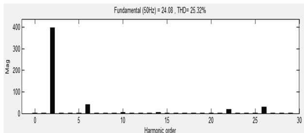
Fig. 10 THD result of 7- Level CHBMLI using MCPWM
