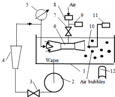
Fig. 1 Experimental setup
