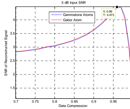
Fig. 14 Matching Pursuit Reconstruction SNR Verses Data Compression for a 5dB SNR
