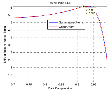
Fig. 15 Matching Pursuit Reconstruction SNR Verses Data Compression for a 10 dB SNR
