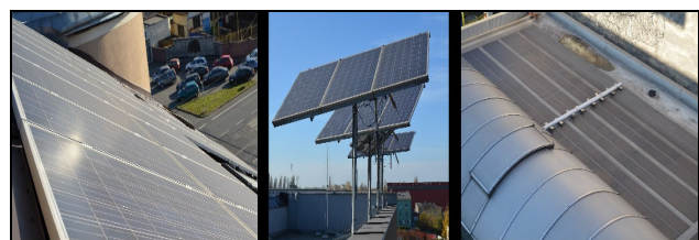
Fig. 3 Three type of photovoltaic panel on the roof of TCO – static panel, tracker and amorphous cells
