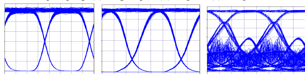
(a) Q = 34.6 dB (b) Q = 38.4 dB (c) Q = 6 dB
