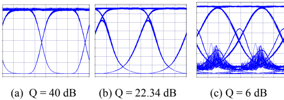
Fig. 6 Eye diagrams for single pumping input 1550 nm, (a) single span (b) 5 spans (c) 8 spans
