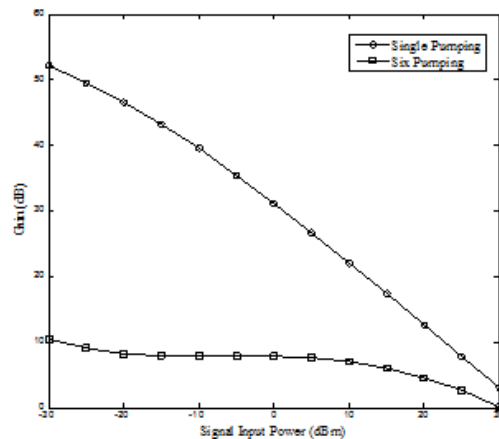
Fig. 11 Variation of Raman gain for five spans of Raman fiber length of 10 km
