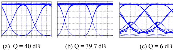
Fig. 7 Eye diagrams for single pumping input 1575 nm, (a) single span (b) 5 spans (c) 8 spans
