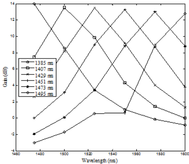
Fig. 1 Gain contribution from individual pump wavelengths
