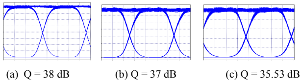
Fig. 8 Eye diagrams for six pumping input 1550 nm, (a) single span (b) 5 spans (c) 8 spans
