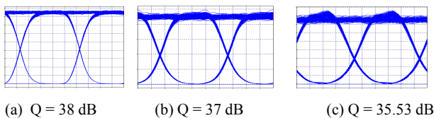
Fig. 9 Eye diagrams for six pumping input 1575 nm, (a) single span (b) 5 spans (c) 8 spans
