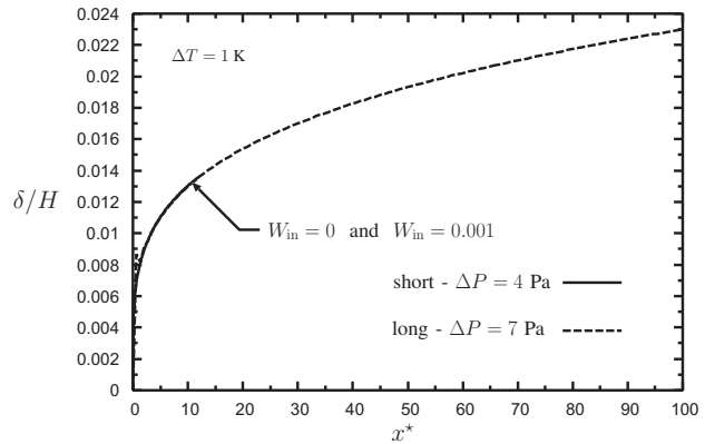
Fig. 2 Film thickness
