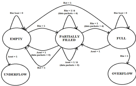
Fig. 5 FIFO state diagram
