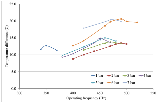
Fig. 2 Temperature difference across the stack versus mean pressure and frequency
