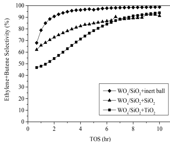
Fig. 4 Ethylene+Butene products selectivity for 10 h time-on-stream
