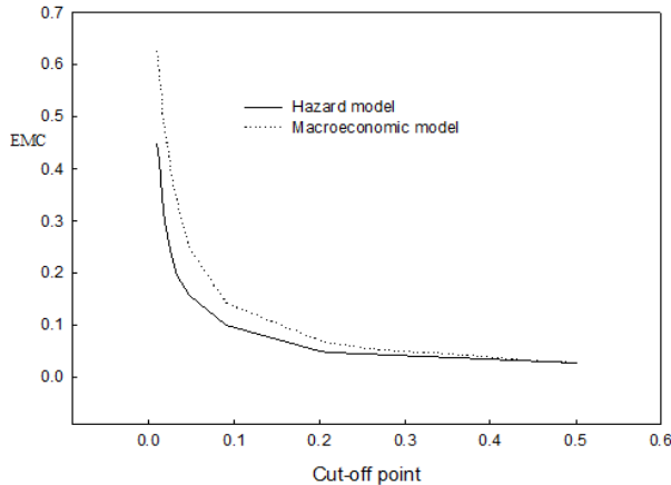
Fig. 1 EMC comparison between hazard models and macroeconomic models for test sample in 2007
