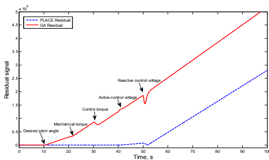
Fig. 8 Incipient actuator fault detection residuals by using the optimal and non-optimal observer gains
