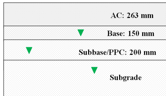
Fig. 2 Elevations of the installed moisture probes
