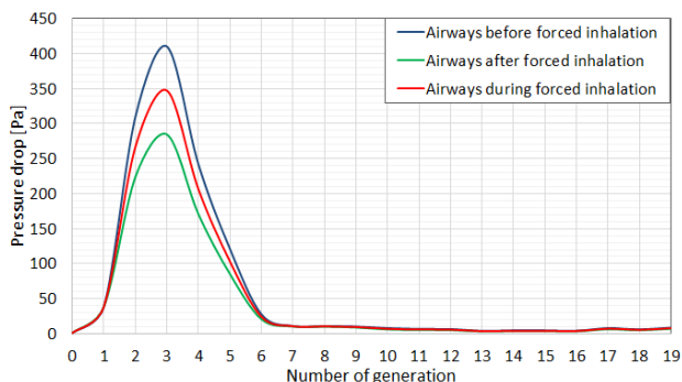
Fig. 10 Pressure drop in the airways during forced inhalation
