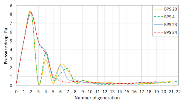
Fig. 5 Pressure drop in the longest airways of BPS 20, 4, 23, 24.
