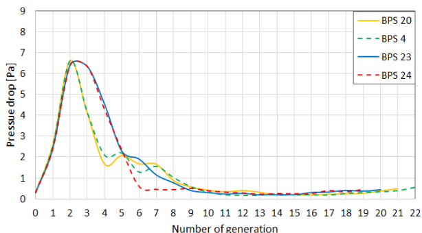
Fig. 6 Pressure drop in the longest airways of BPS 20, 4, 23, 24 after correction
