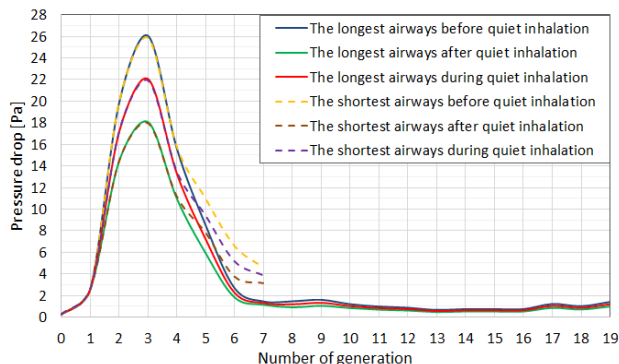
Fig. 9 Pressure drop in the airways during quiet inhalation in the longest and the shortest airway in BPS 24
