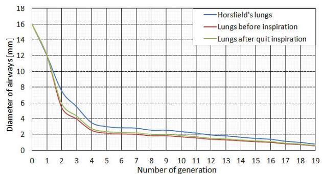
Fig. 4 Dimensions of the airways
