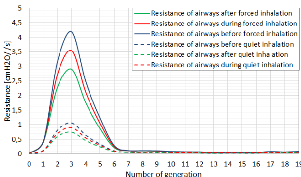
Fig. 14 Resistance of airways
