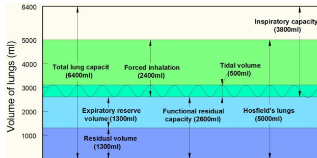
Fig. 3 Capacity of Horsfield's lung
