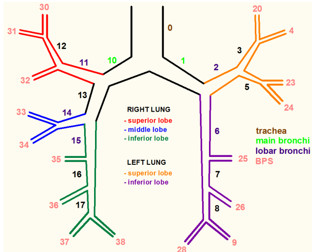
Fig. 2 Horsfield's model of human bronchial tree
