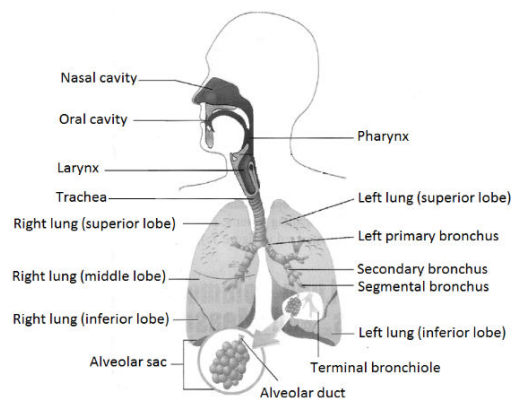
Fig. 1 Morphology of human lungs [3]
