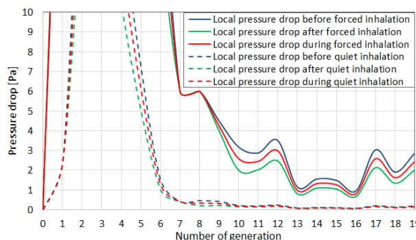
Fig. 12 Local pressure drop in the airways during quit and forced inhalation - detail the terminal bronchiole
