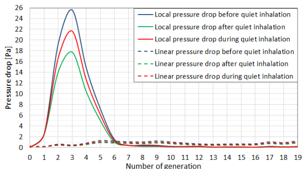
Fig. 8 Local and linear pressure drop in the airways during quiet inhalation
