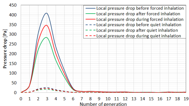
Fig. 11 Local pressure drop in the airways during quit and forced inhalation
