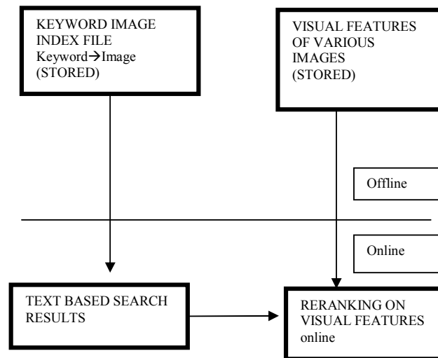
Fig. 1 Earlier Image Re-ranking Framework
