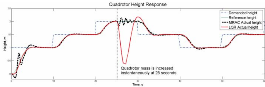
Fig. 4. Simulation of Quadrotor Height Response
