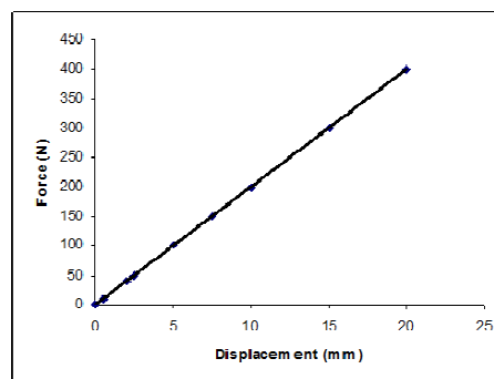
Fig. 3 Calibration curve of the burnishing tool spring
