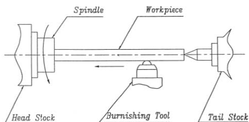
Fig. 4 Set-up of a ball burnishing process [8]
