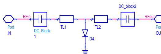
Fig. 1 Power Limiter topology
