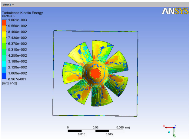
Fig. 7 Turbulence K.E. contour of initially designed fan
