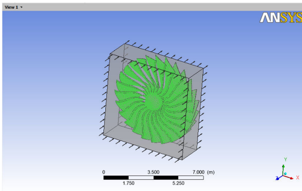
Fig. 3 Computational domain of fan
