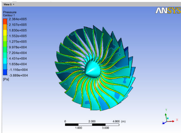
Fig. 6 Pressure contour of fan
