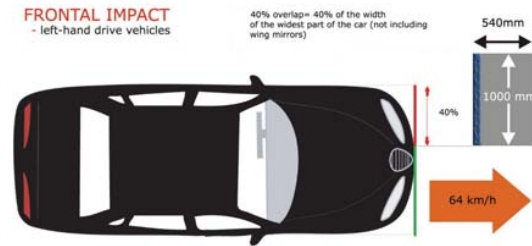
Fig. 4: Frontal impact Euro-NCAP [6]
