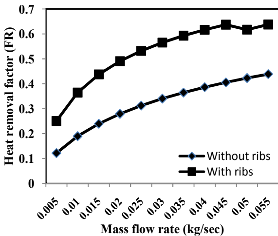
Fig. 6 Variation of heat removal factor with respect to mass flow rate of air
