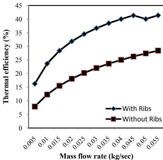
Fig. 5 Variation of thermal efficiency with respect to mass flow rate of air
