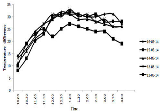
Fig. 9 Variation of temperature in rough solar collector with respect to time
