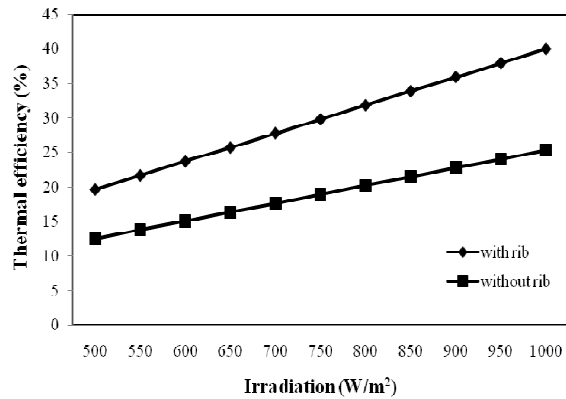
Fig. 4 Variation of thermal efficiency with respect to irradiation
