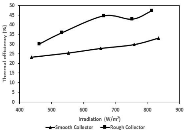
Fig. 7 Variation in thermal efficiency with respect to irradiation of smooth and rough solar collector
