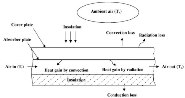
Fig. 1 Energy balance of solar air heater [16]
