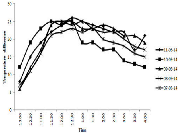
Fig. 8 Variation of temperature in smooth solar collector with respect to time
