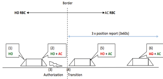
Fig. 5 Example of RBC-RBC Handover Scenario
