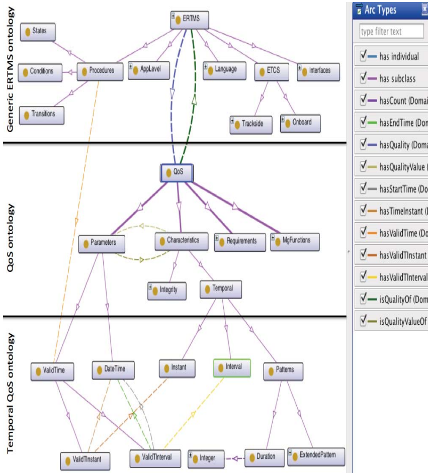
Fig. 4 3-Layer Temporal QoS Ontology for ERTMS/ETCS
