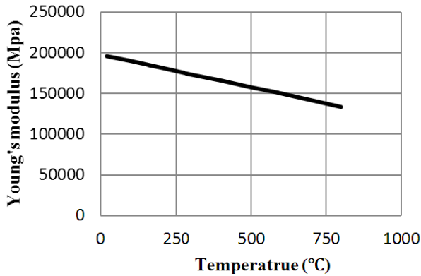
Fig. 4 Relation between young's modulus and temperature
