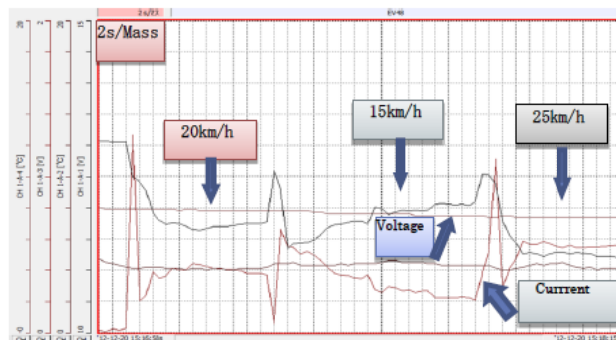
Fig. 6 Battery voltage, current and temperature during driving
