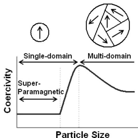
Fig. 1 Variation of coercivity with particle size
