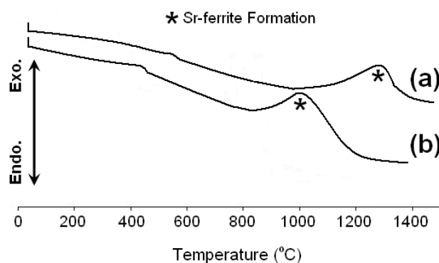
Fig. 3 DTA curve of powder obtained by (a) conventional method (b) sol-gel auto-combustion method, before calcination process
