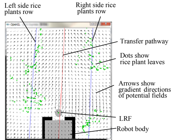
Fig. 2 Graphics of the potential method
