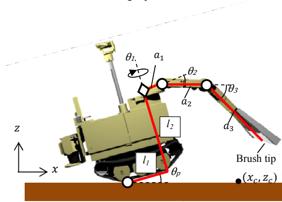
Fig. 7 Parameters for posture control of the robot arm
