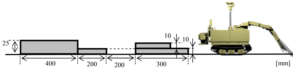
Fig. 8 Posture control preliminary experiment
