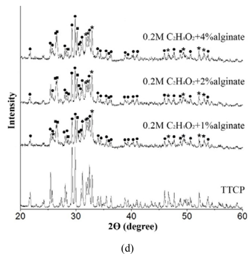
Fig. 1 XRD patterns of TTCP and CPC with (a) \text{Na}_2\text{HPO}_4 \cdot 2\text{H}_2\text{O} , (b) \text{C}_2\text{H}_4\text{O}_2 , (c) 0.2M \text{Na}_2\text{HPO}_4 \cdot 2\text{H}_2\text{O} +alginate and (d) 0.2M \text{C}_2\text{H}_4\text{O}_2 +alginate ; * HA, ● TTCP, ■ DCPA
