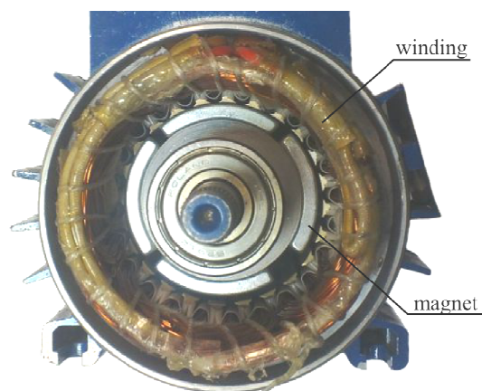
Fig. 4 PM machine
