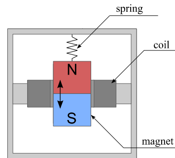
Fig. 3 An electrodynamic sensor
