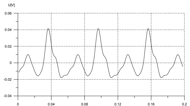
Fig. 7 The waveform of the induced emf - the result of simulation
