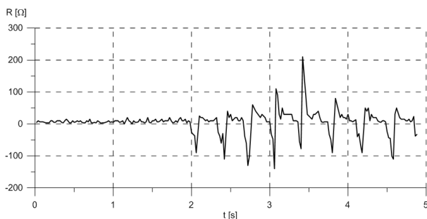
Fig. 2 Distortions during the resistance measurements
