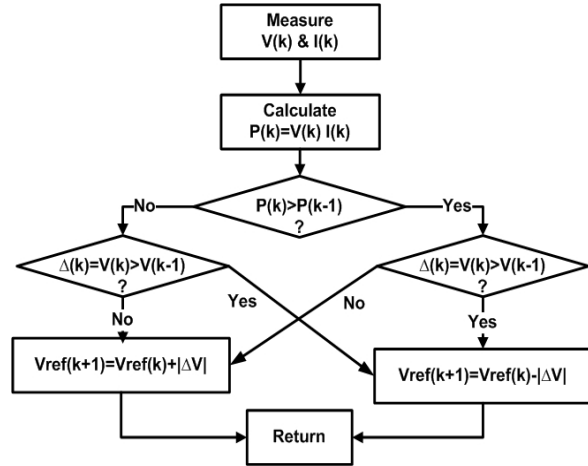
Fig. 2 P&amp;O MPPT algorithm
