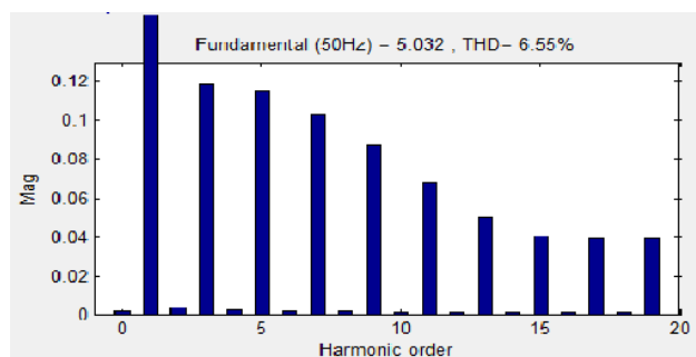
Fig. 10 FFT Analysis of Hybrid Rectifier
