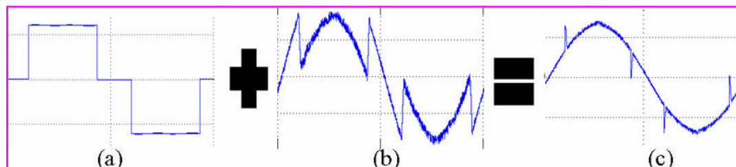
Fig. 8 Simulated Current Waveform of Hybrid Rectifier (a) Current wave form imposed by the ZVT- ZCT switch boost rectifier (Uncontrolled Rectifier) (b) Injected Current wave form generator by six pulse boost rectifier (Controlled Rectifier) (c) Desired sinusoidal waveform
