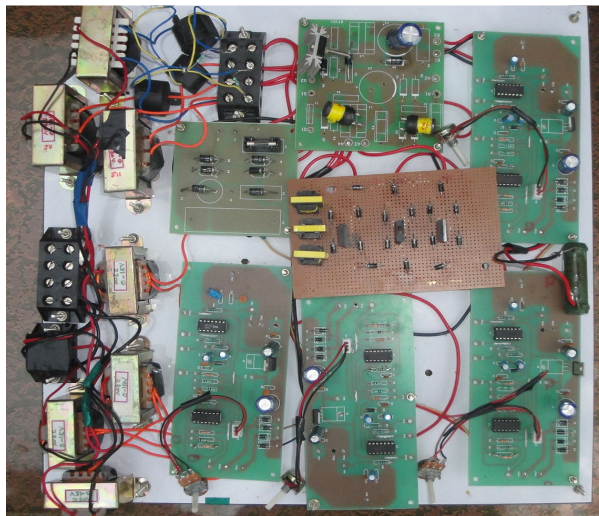
Fig. 13 Prototype of Hybrid Rectifier
