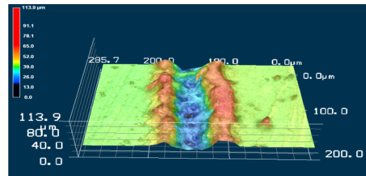
(a) Laser power 5 W
