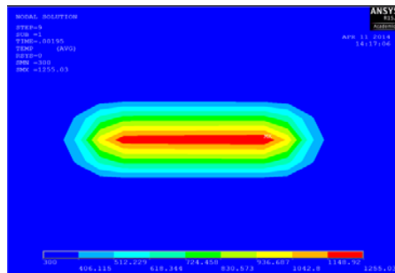
(b) The laser power 12 W
