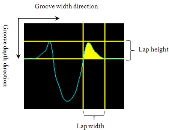
Fig. 8 The groove dimensions (width and the height)
