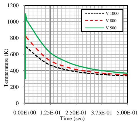
(b) The effect of the laser speed on the temperature variation at point ( y= 0, x =6.3 mm) and p 17 (W)
