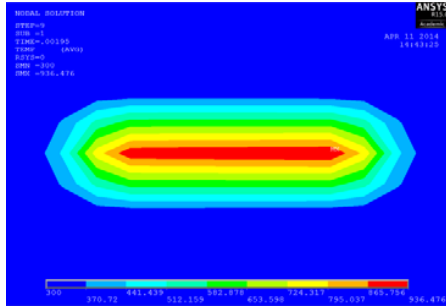
(a) The laser power 8 W
