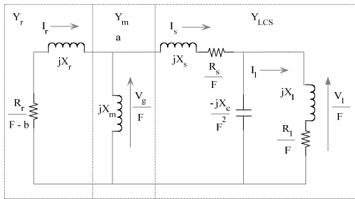
Fig. 1 Per phase equivalent circuit of SEIG
