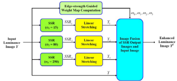
Fig. 1 Flow diagram of the proposed EGMSR approach
