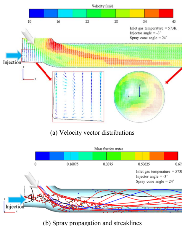
Fig. 4 Numerical results at xz cross section of the exhaust pipe. The spray conditions are injector angle of -3^\circ and spray cone angle of 24^\circ at inlet gas temperature of 573K ( t=0.7\text{s} ): (a) Velocity vector distributions, (b) Spray propagation (droplets are colored with water fraction) and streaklines
