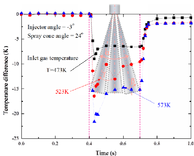
Fig. 3 Effect of inlet gas temperature on the temperature difference. The spray conditions are injector angle of -3^\circ and spray cone angle of 24^\circ
