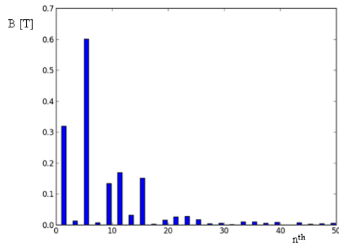
Fig. 16 FFT of the average magnetic flux density in rotor teeth of the optimized motor
