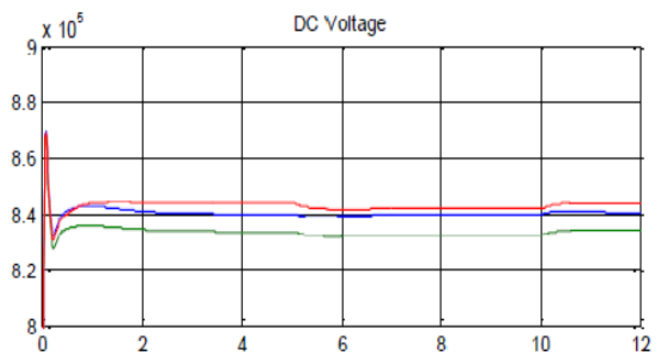
Fig. 13 (b) 3 Terminal MTDC with changed Voltage and Power References
